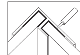
External corner Used on all external 90° corners
