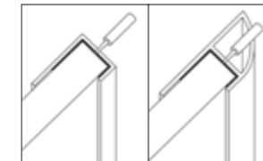
End & Quadrant Trims Finishing end trims for panels
